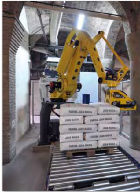
Side grip, valve bags
