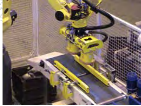
Grip by vacuum
