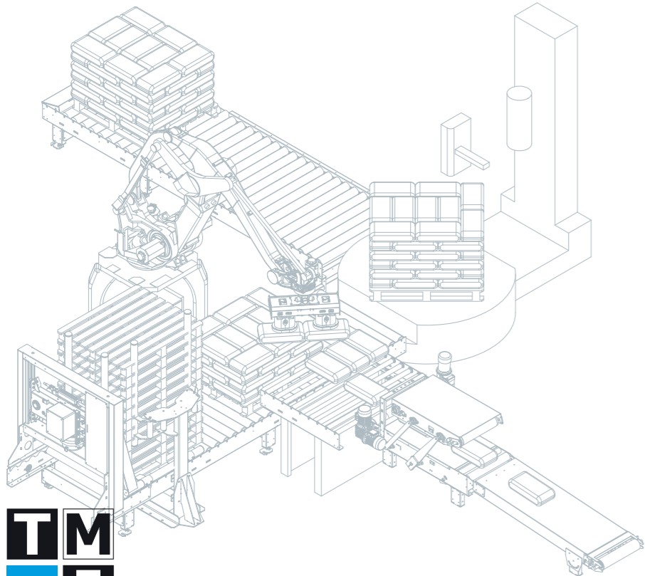
Versatile grips for cases, bags and pallets.
