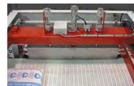
Special belts for bag sliding
